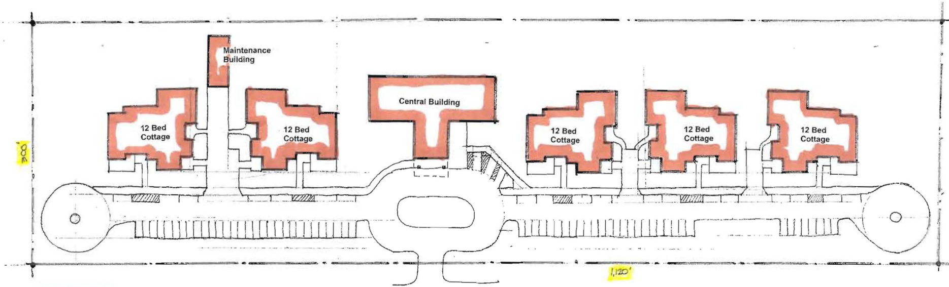
Cottage Model Campus-Linear Layout Scale: 0 10 50 100'
